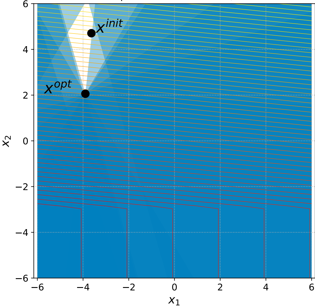
17 Linear Slope with 6+n constraints, instance=4
