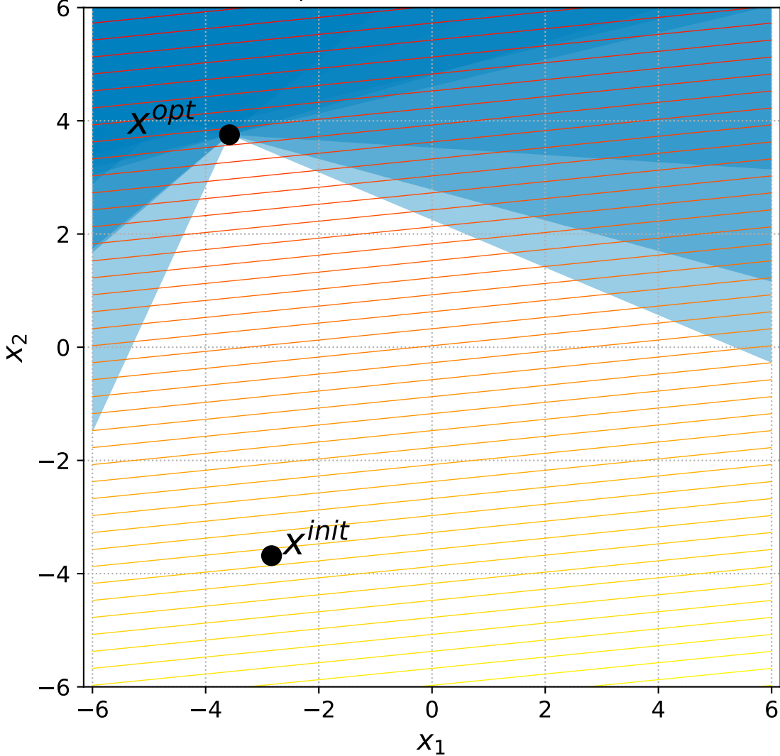
17 Linear Slope with 6+n constraints, instance=3
