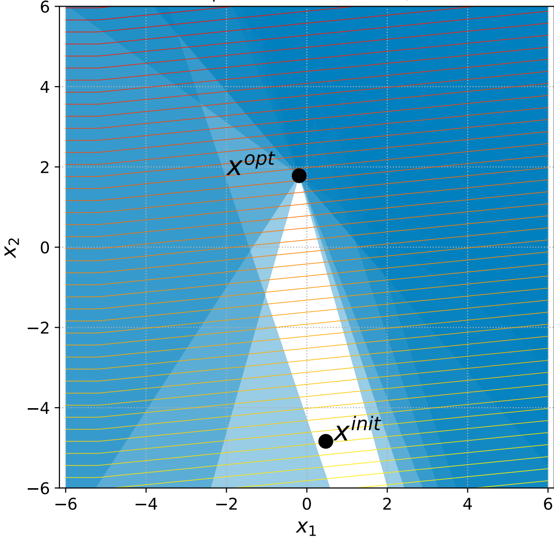
17 Linear Slope with 6+n constraints, instance=2
