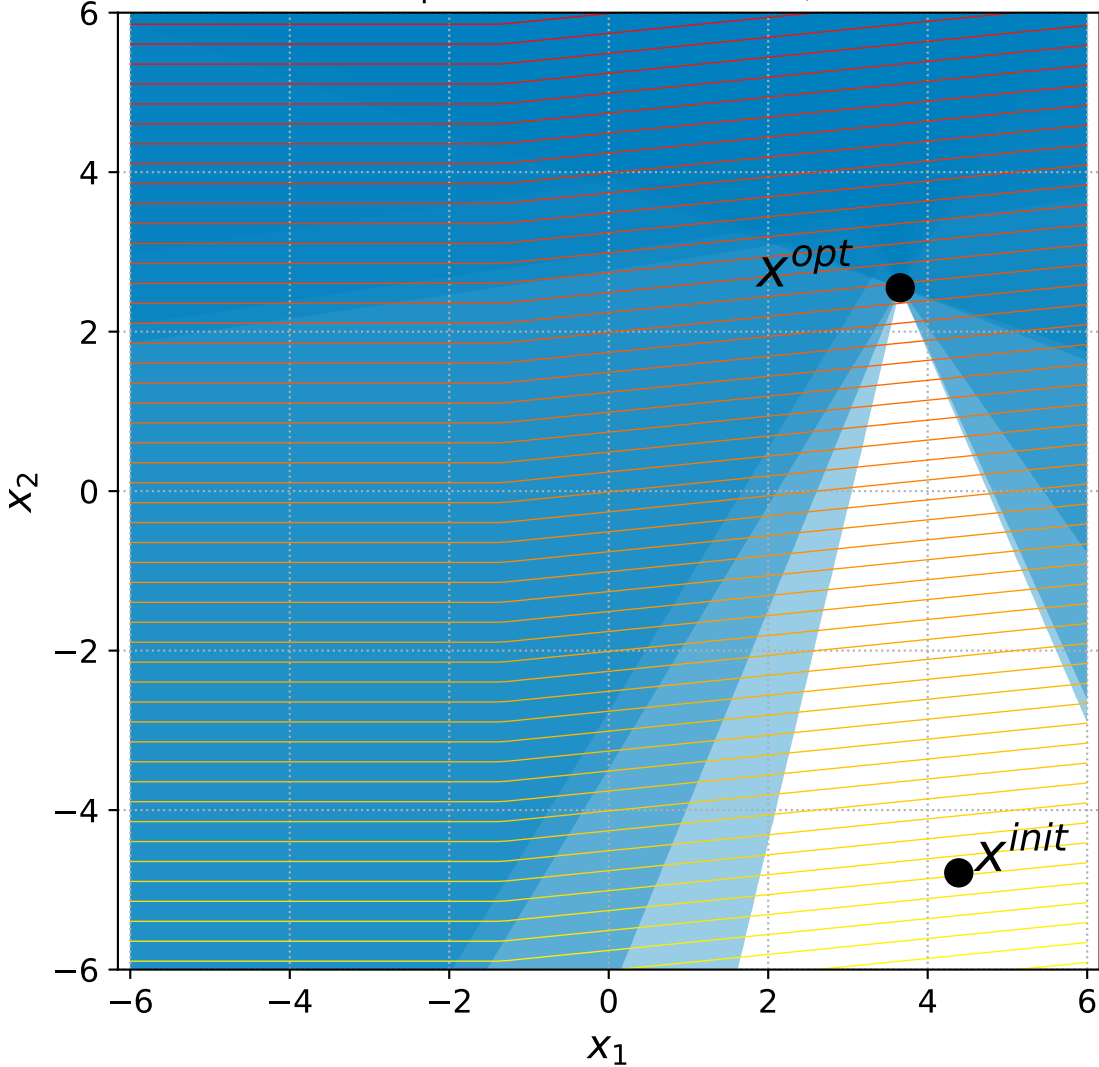
17 Linear Slope with 6+n constraints, instance=1
