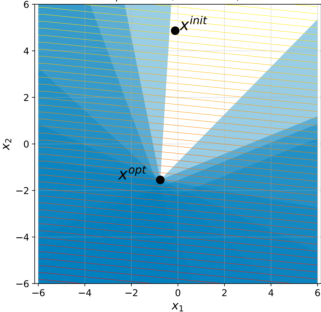
16 Linear Slope with 6+n/2 constraints, instance=15
