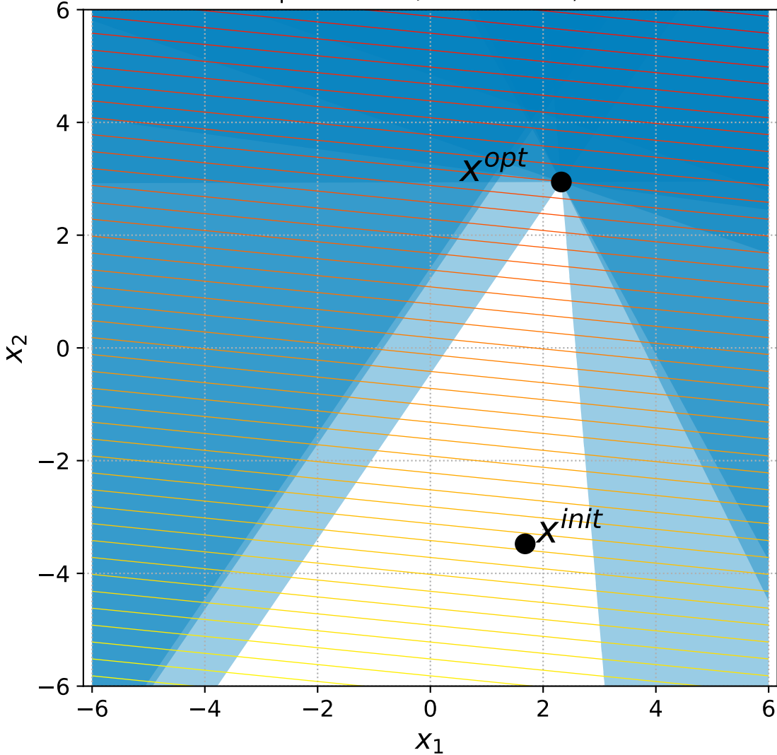
16 Linear Slope with 6+n/2 constraints, instance=13
