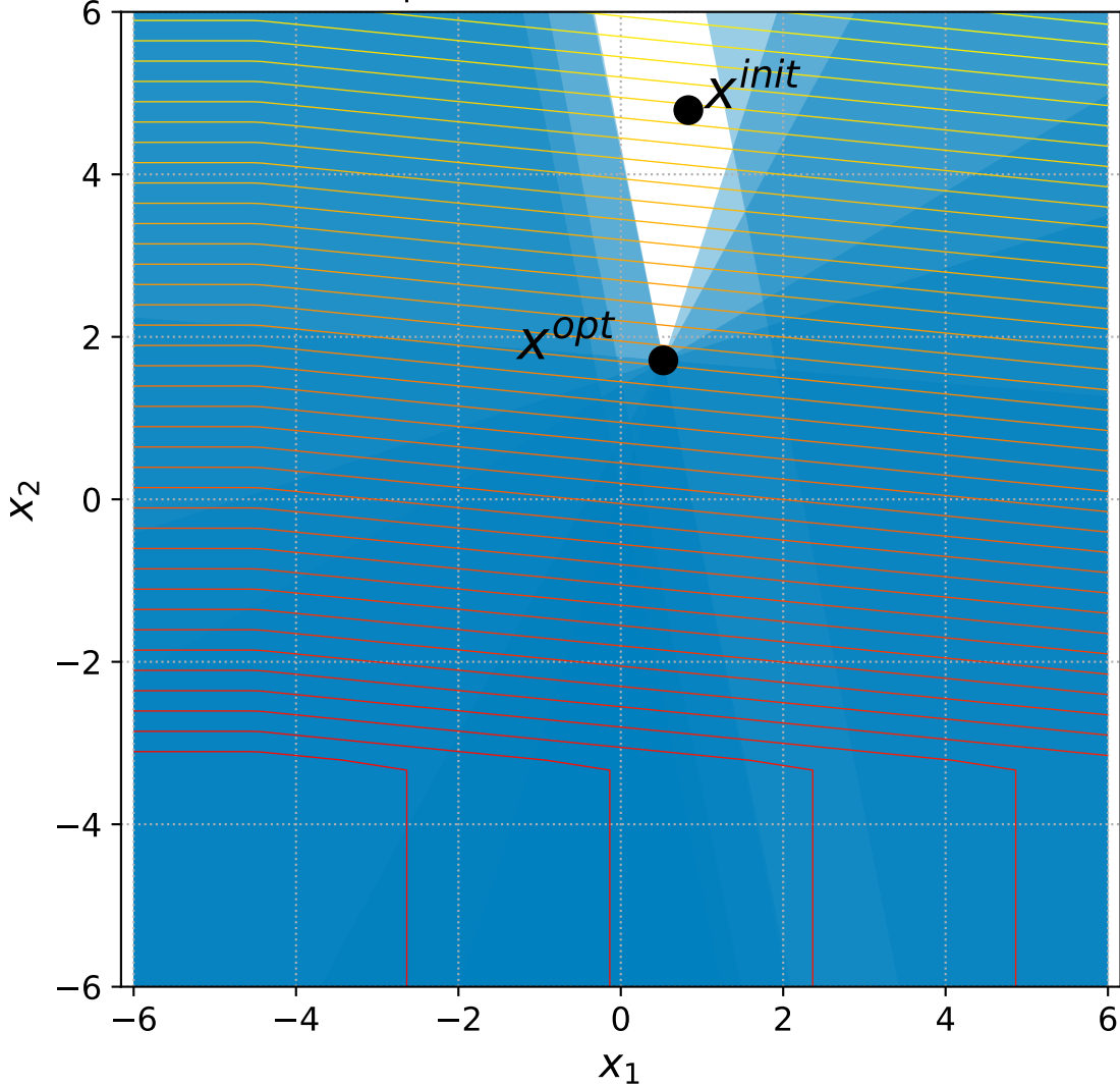
16 Linear Slope with 6+n/2 constraints, instance=12
