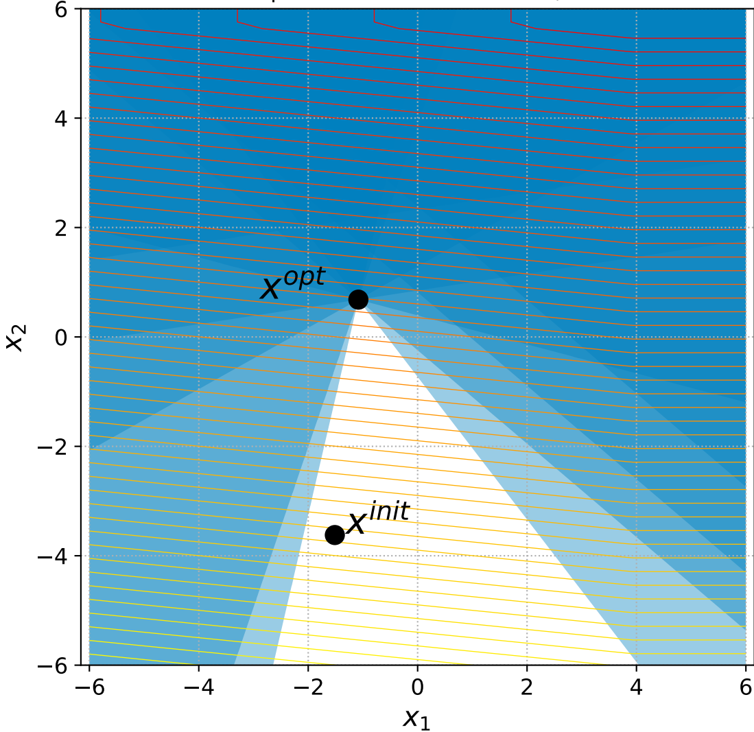
16 Linear Slope with 6+n/2 constraints, instance=11
