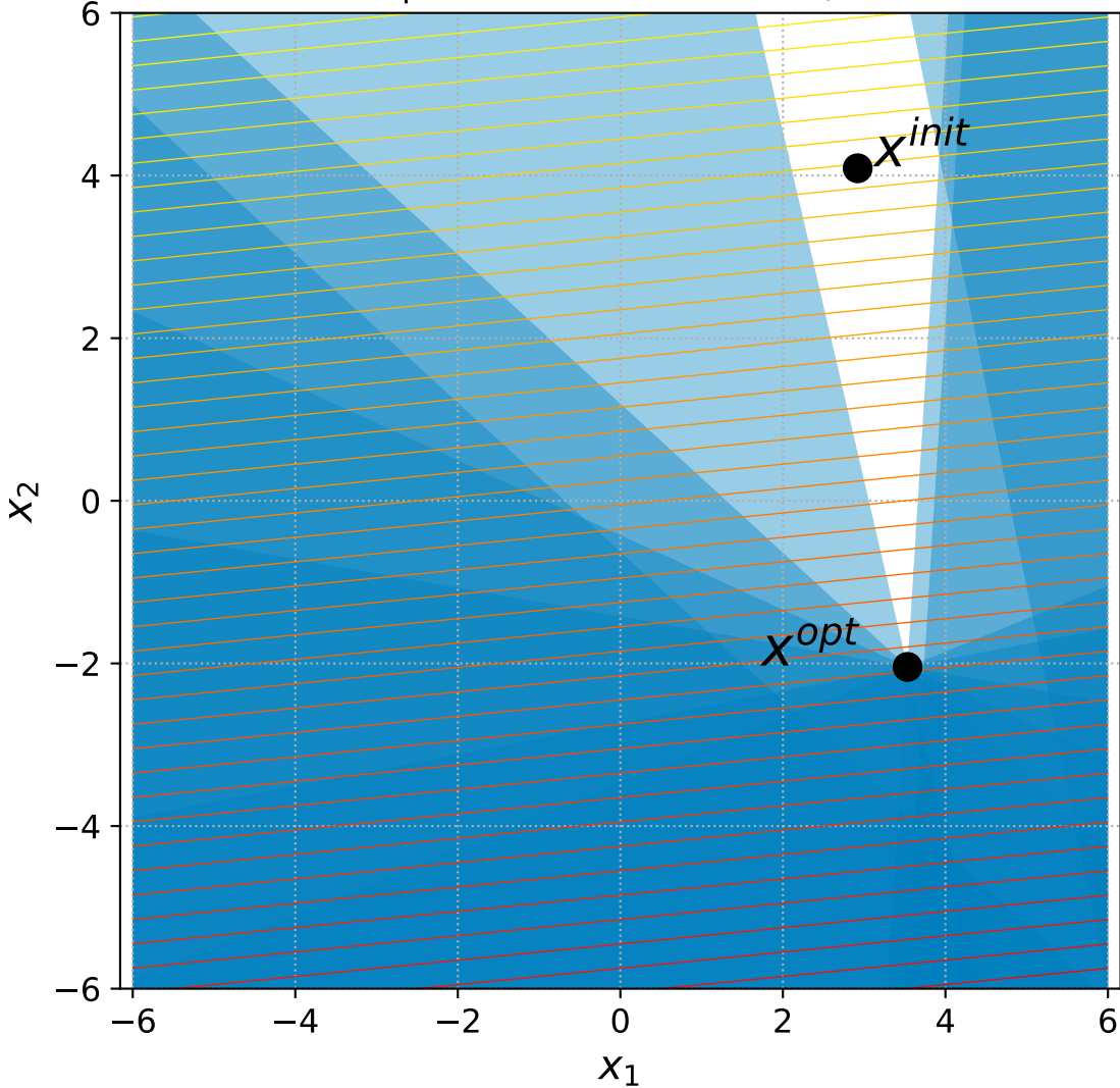
16 Linear Slope with 6+n/2 constraints, instance=10
