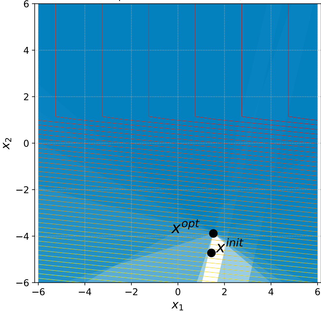
16 Linear Slope with 6+n/2 constraints, instance=6
