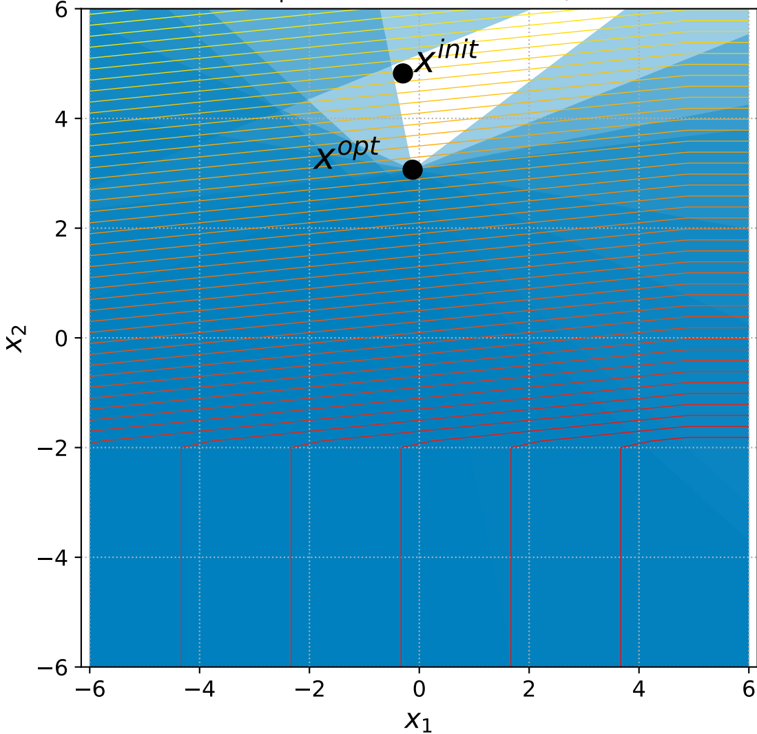
16 Linear Slope with 6+n/2 constraints, instance=5
