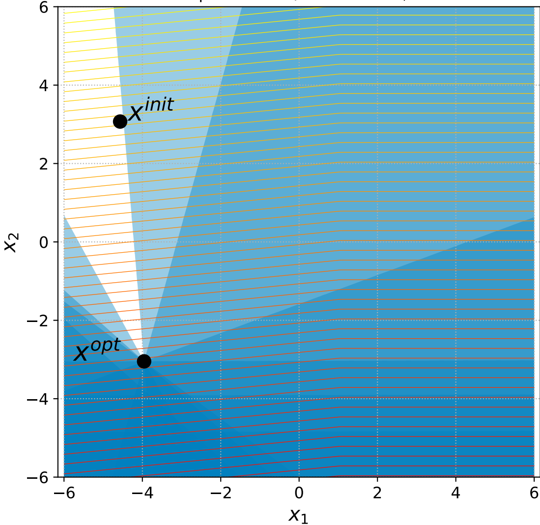
16 Linear Slope with 6+n/2 constraints, instance=3
