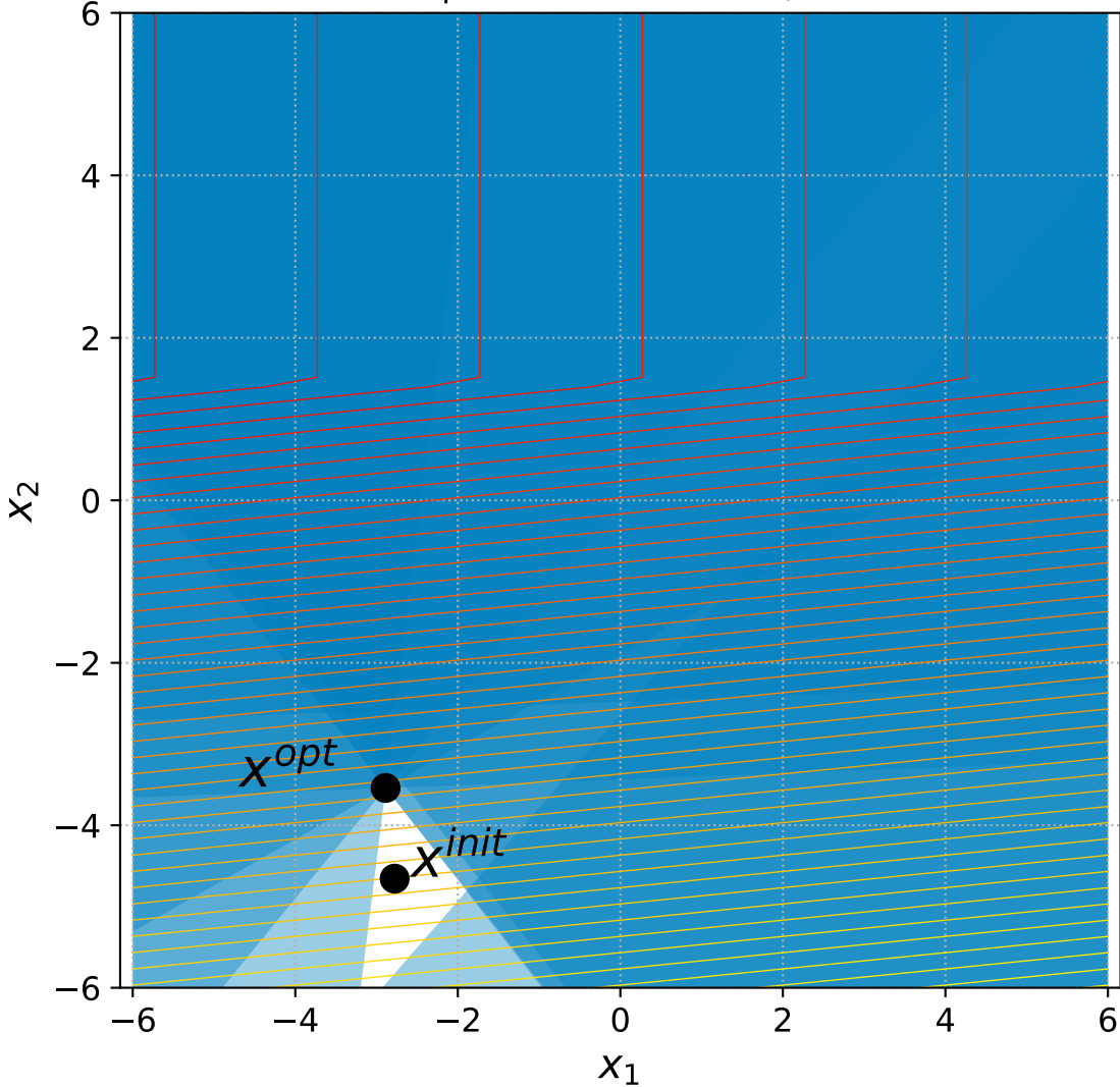
15 Linear Slope with 6 constraints, instance=15
