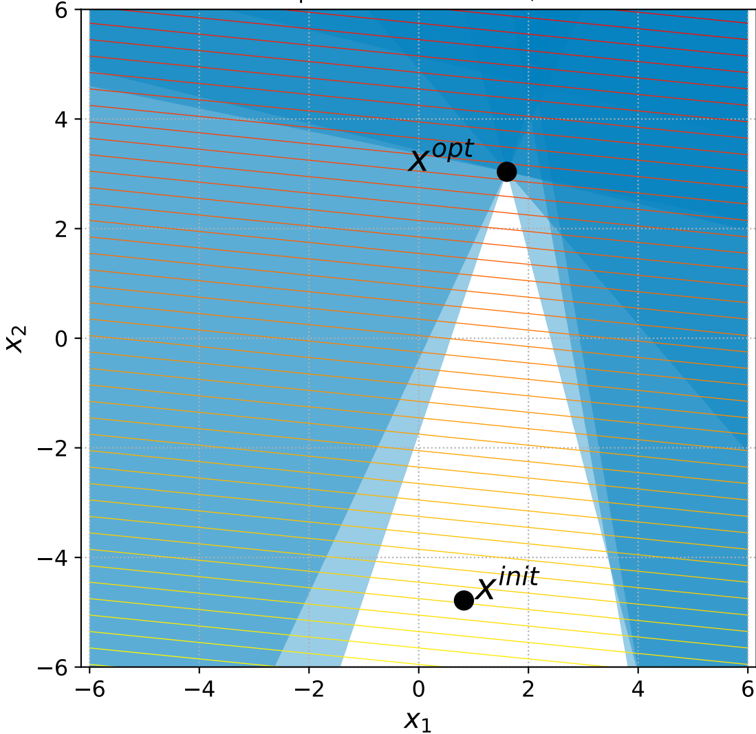
15 Linear Slope with 6 constraints, instance=13
