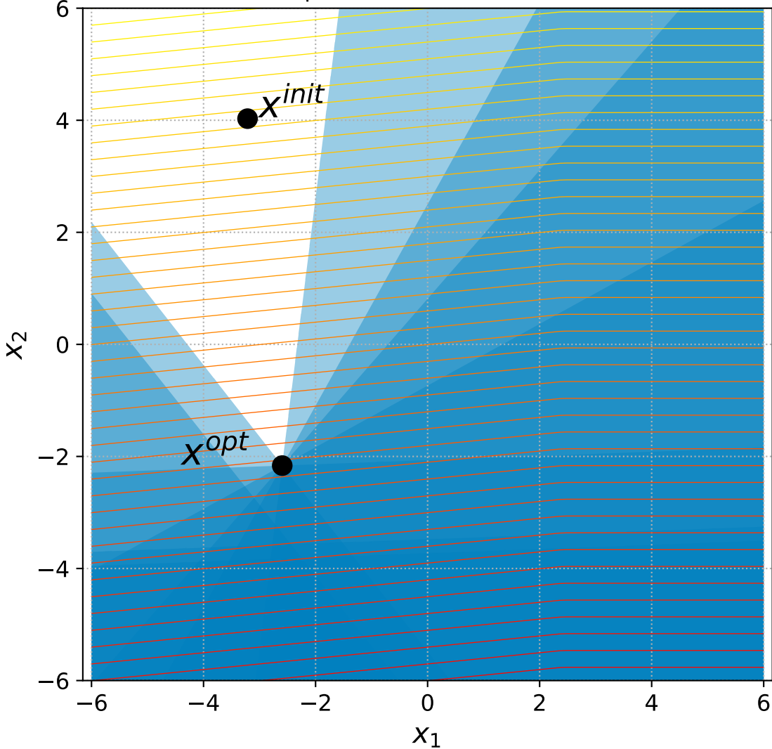
15 Linear Slope with 6 constraints, instance=10
