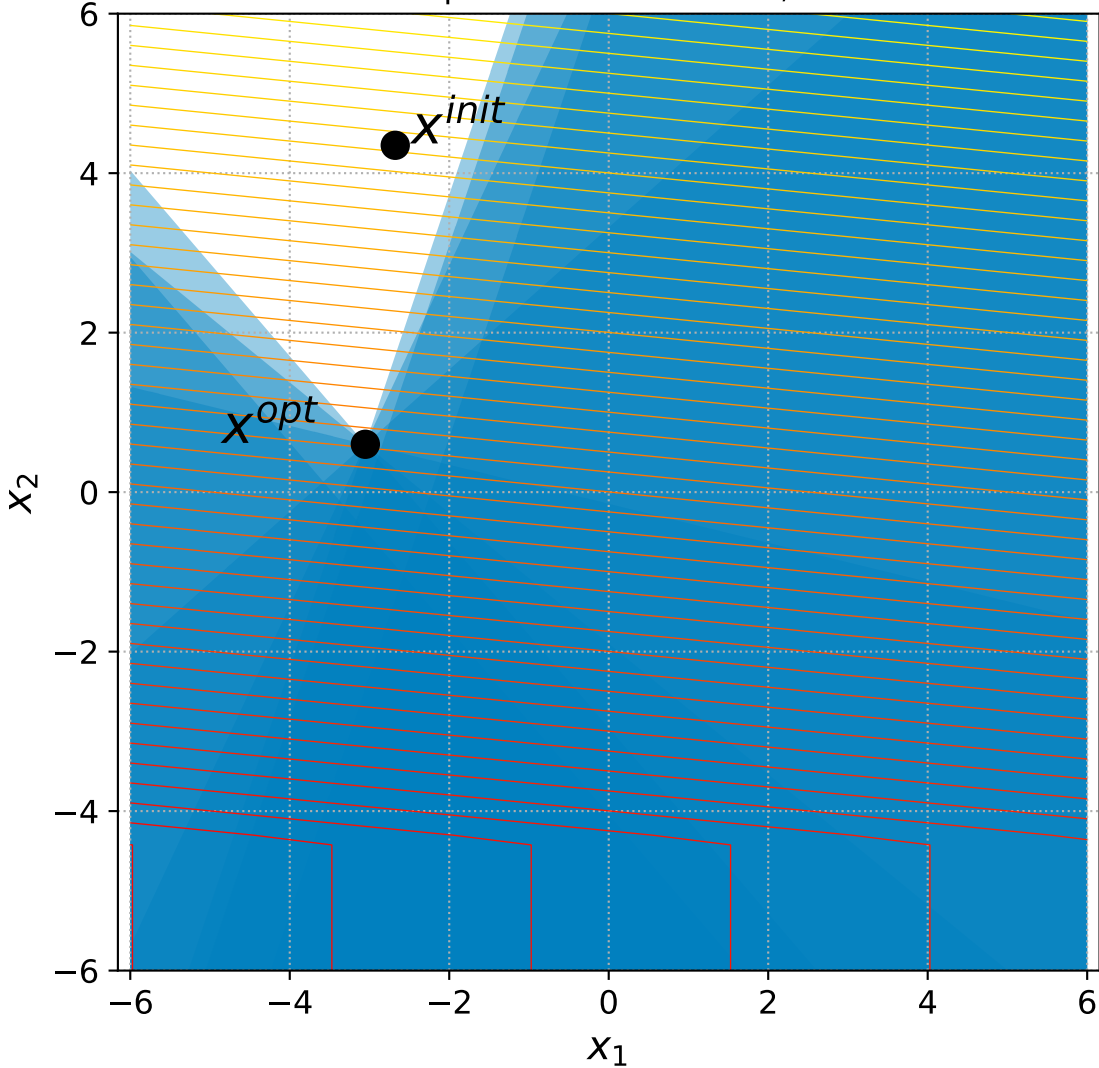
15 Linear Slope with 6 constraints, instance=8
