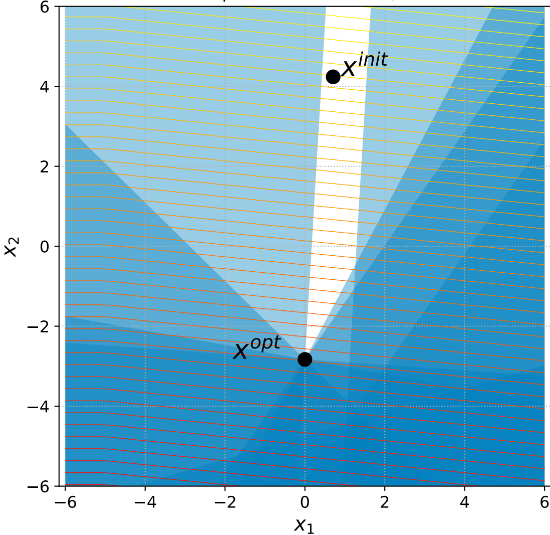
15 Linear Slope with 6 constraints, instance=6
