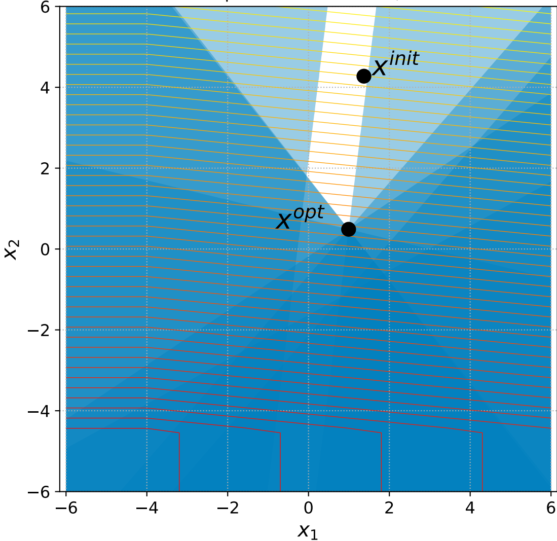
15 Linear Slope with 6 constraints, instance=5
