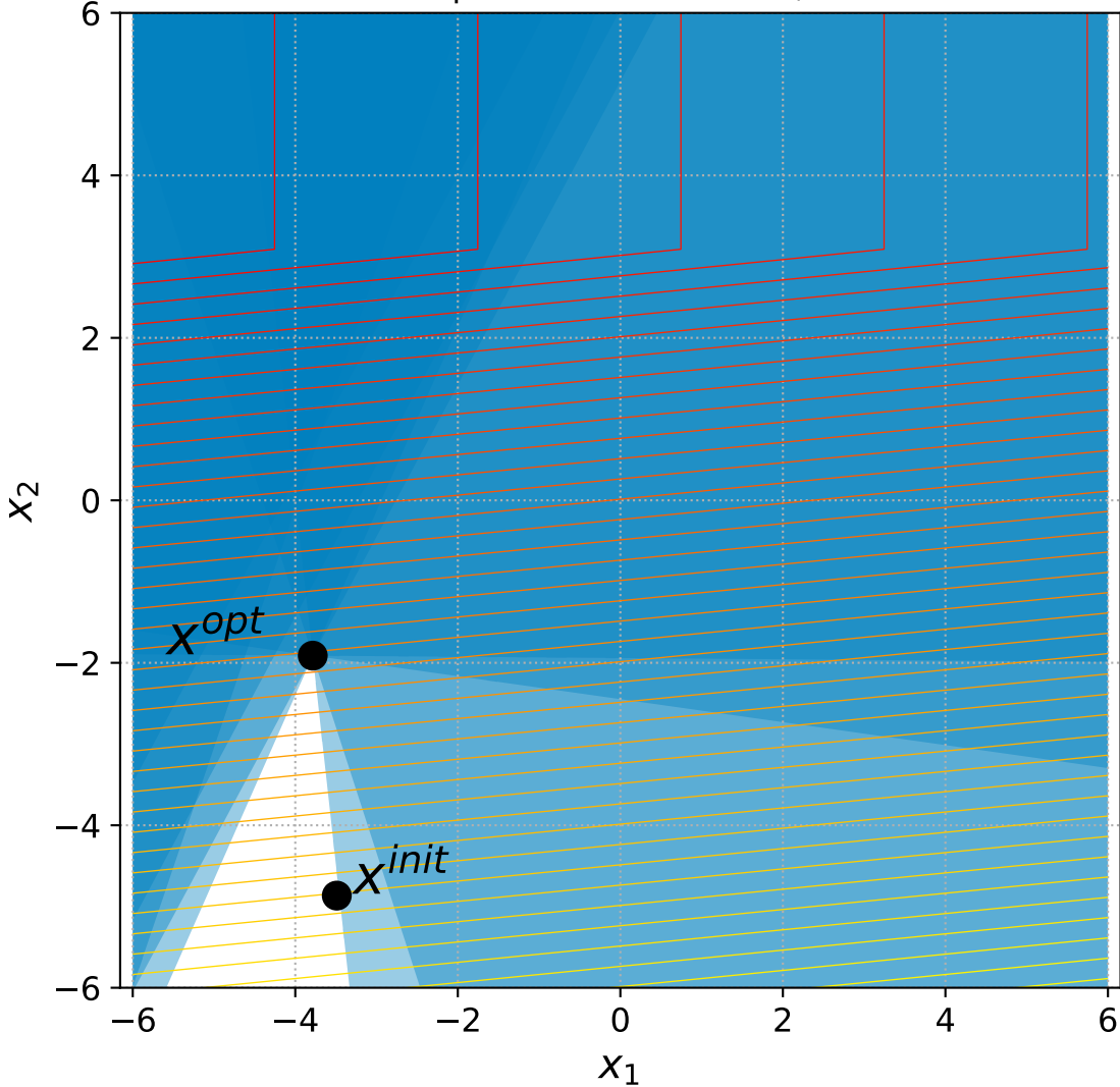
15 Linear Slope with 6 constraints, instance=4
