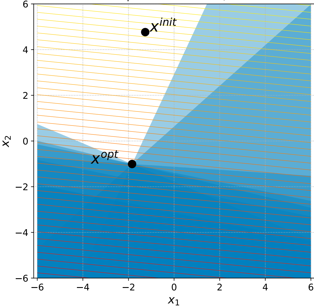
15 Linear Slope with 6 constraints, instance=3
