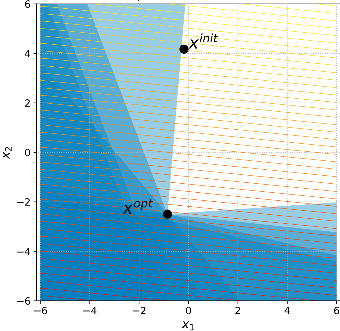
15 Linear Slope with 6 constraints, instance=2
