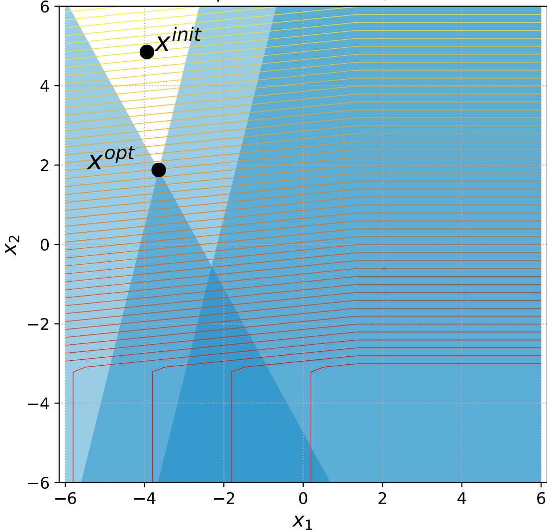
14 Linear Slope with 2 constraints, instance=13
