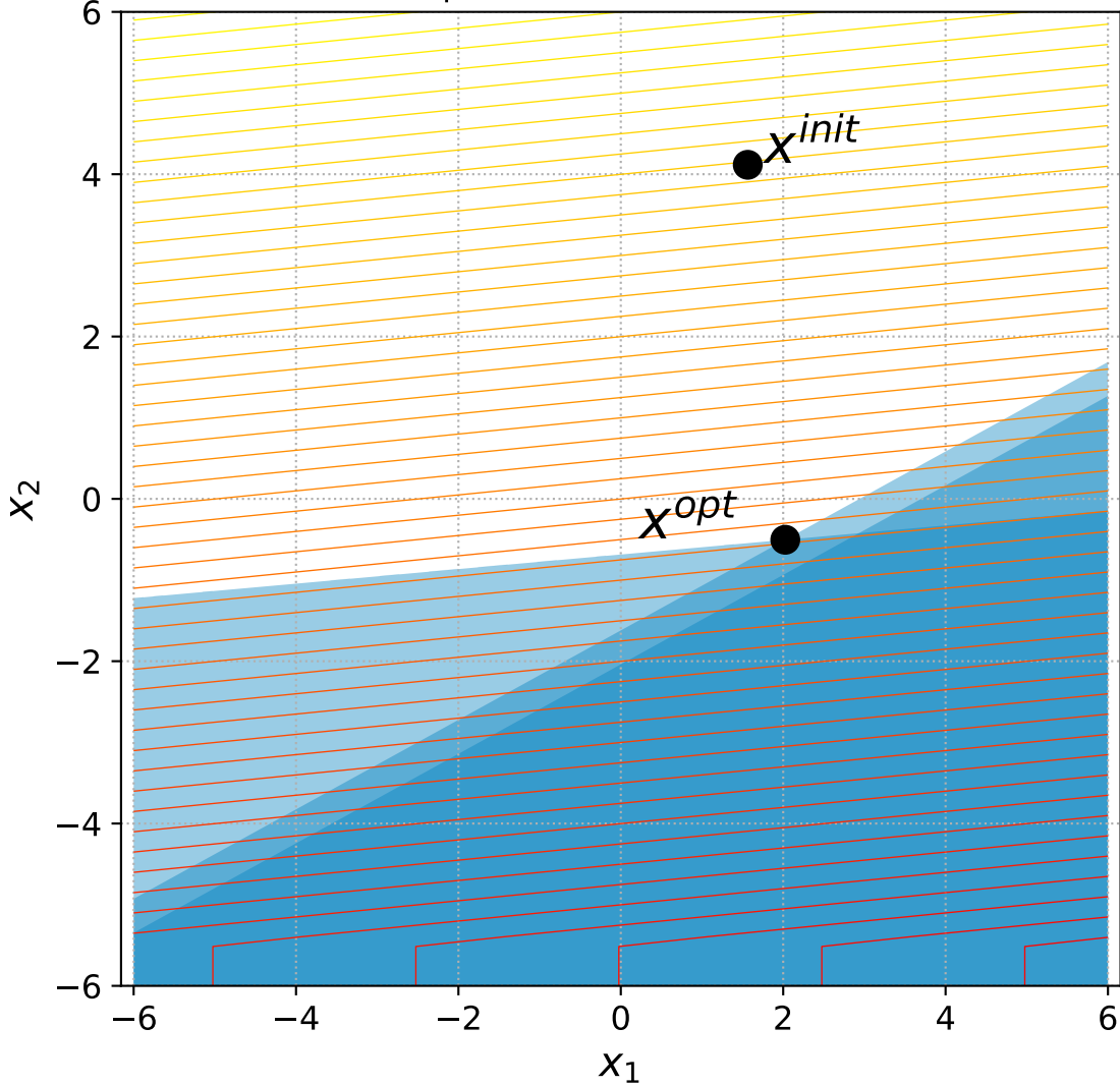
14 Linear Slope with 2 constraints, instance=11
