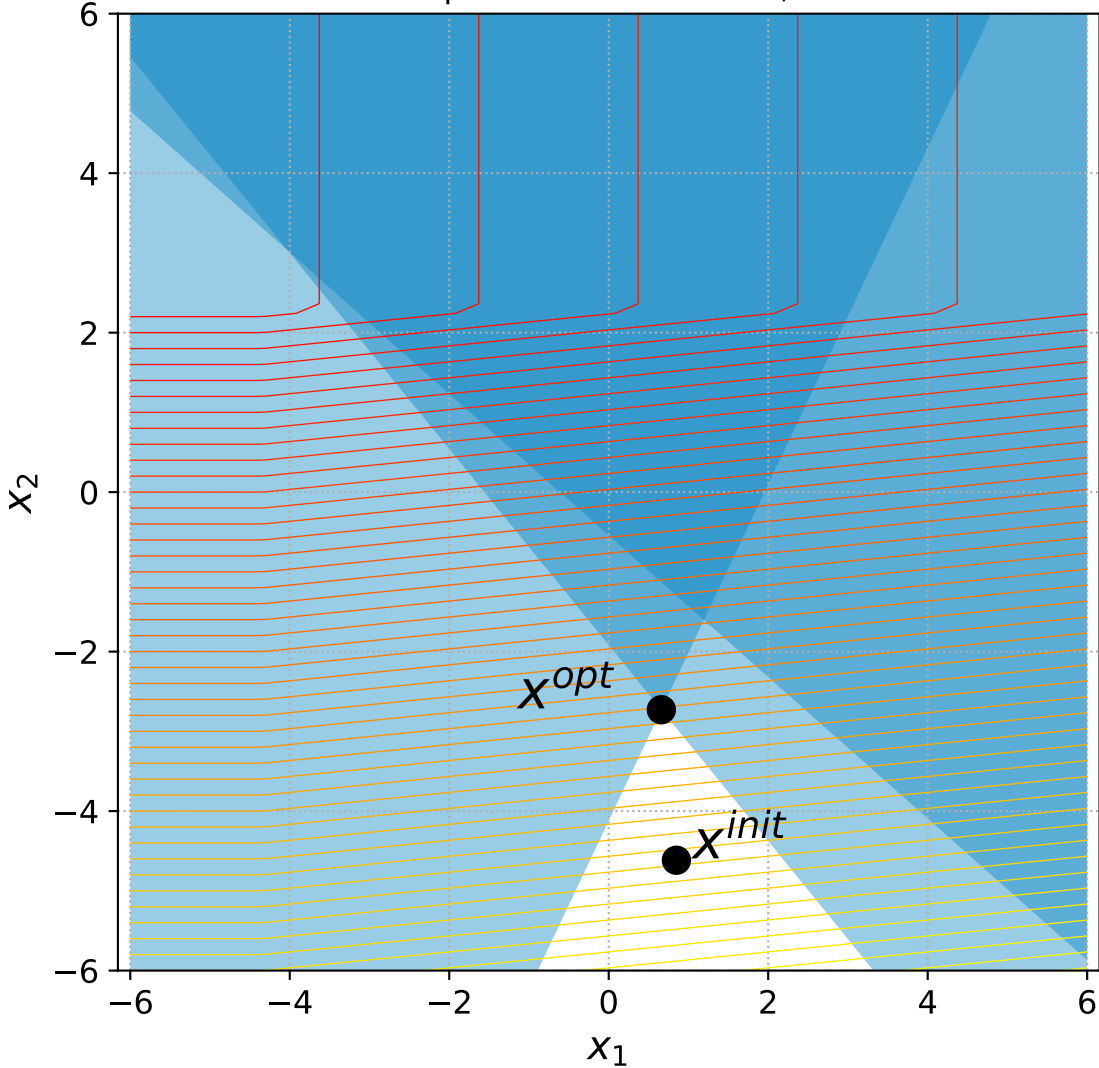
14 Linear Slope with 2 constraints, instance=9
