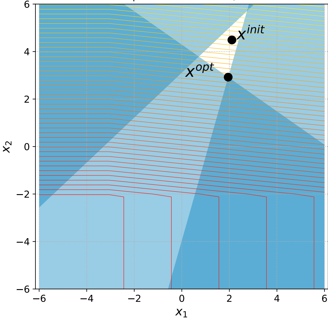
14 Linear Slope with 2 constraints, instance=5
