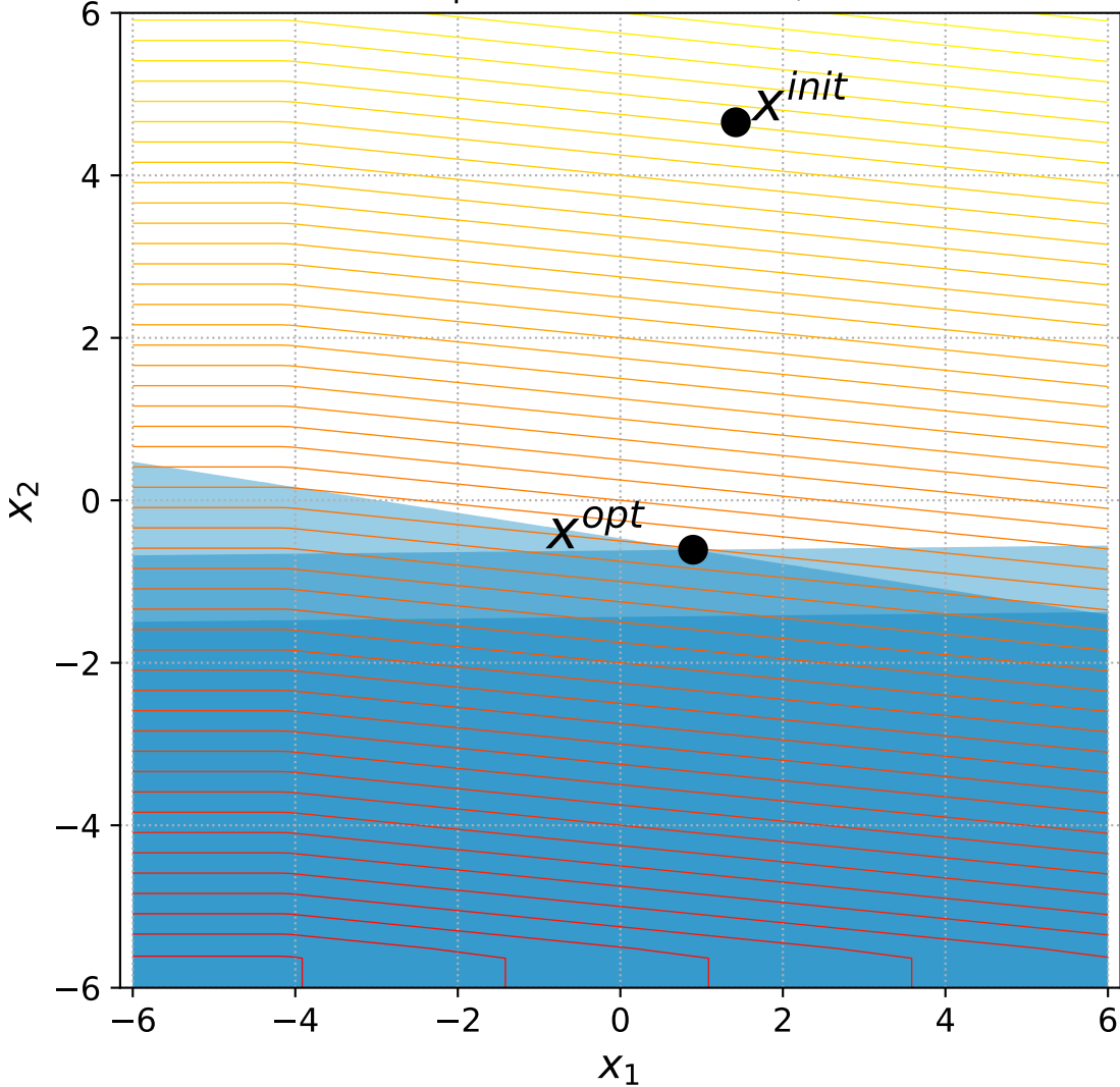
14 Linear Slope with 2 constraints, instance=3
