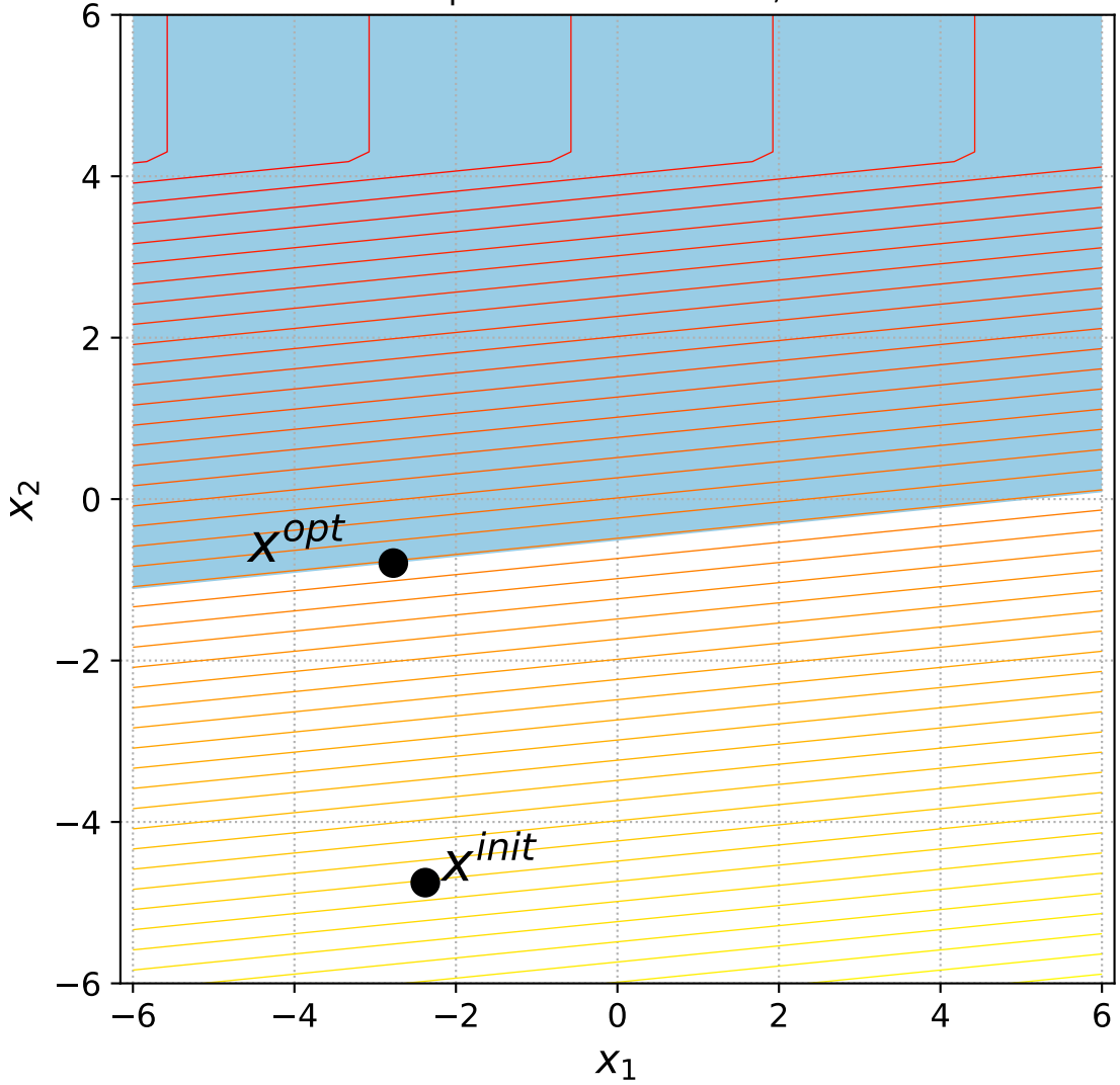
13 Linear Slope with 1 constraint, instance=15
