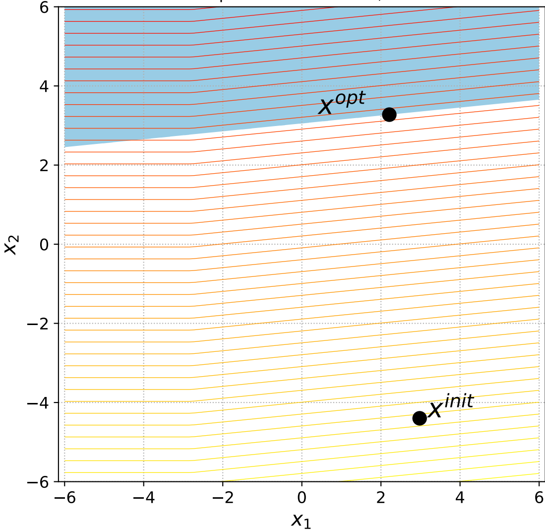
13 Linear Slope with 1 constraint, instance=12
