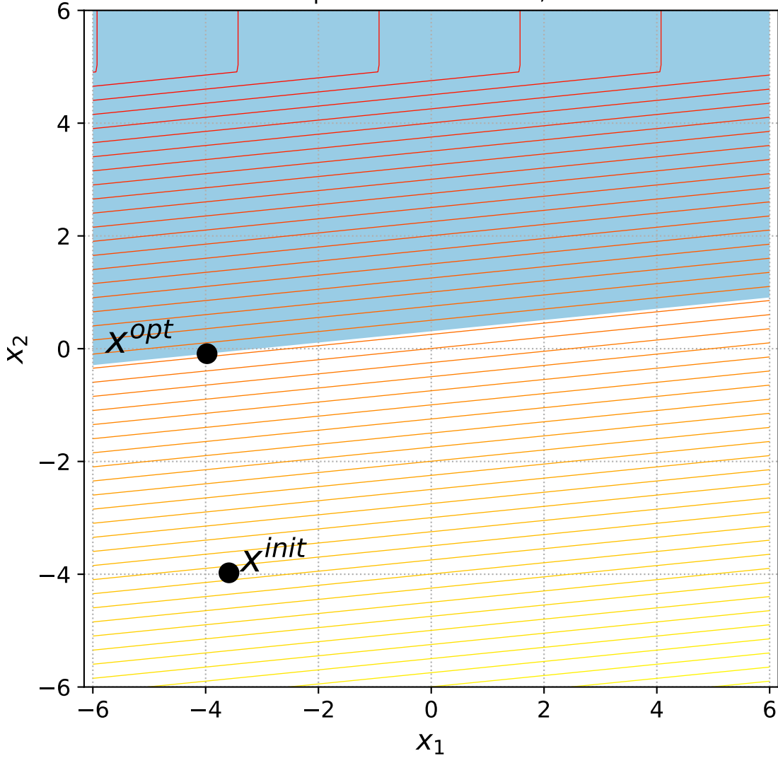
13 Linear Slope with 1 constraint, instance=11
