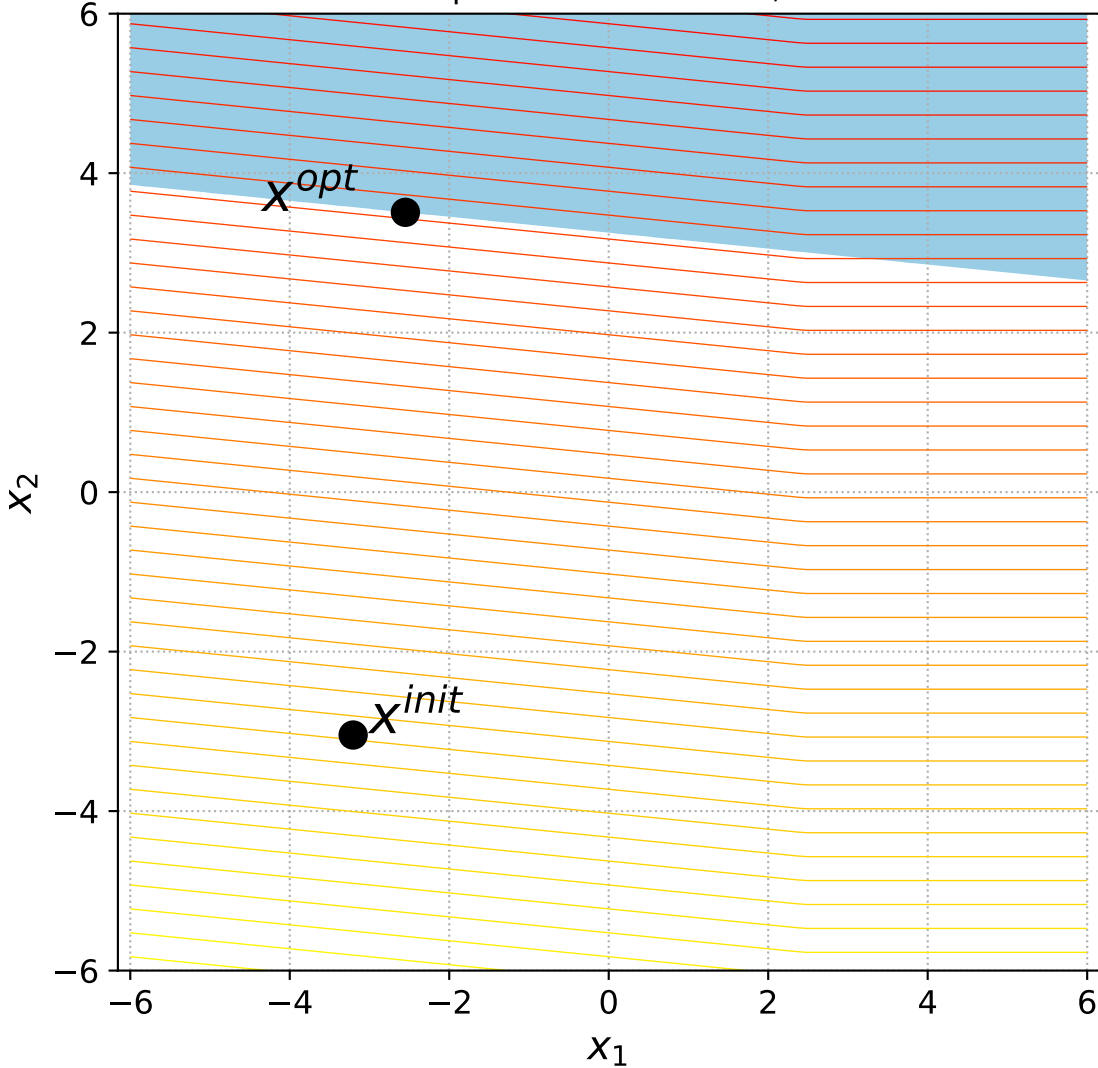
13 Linear Slope with 1 constraint, instance=9
