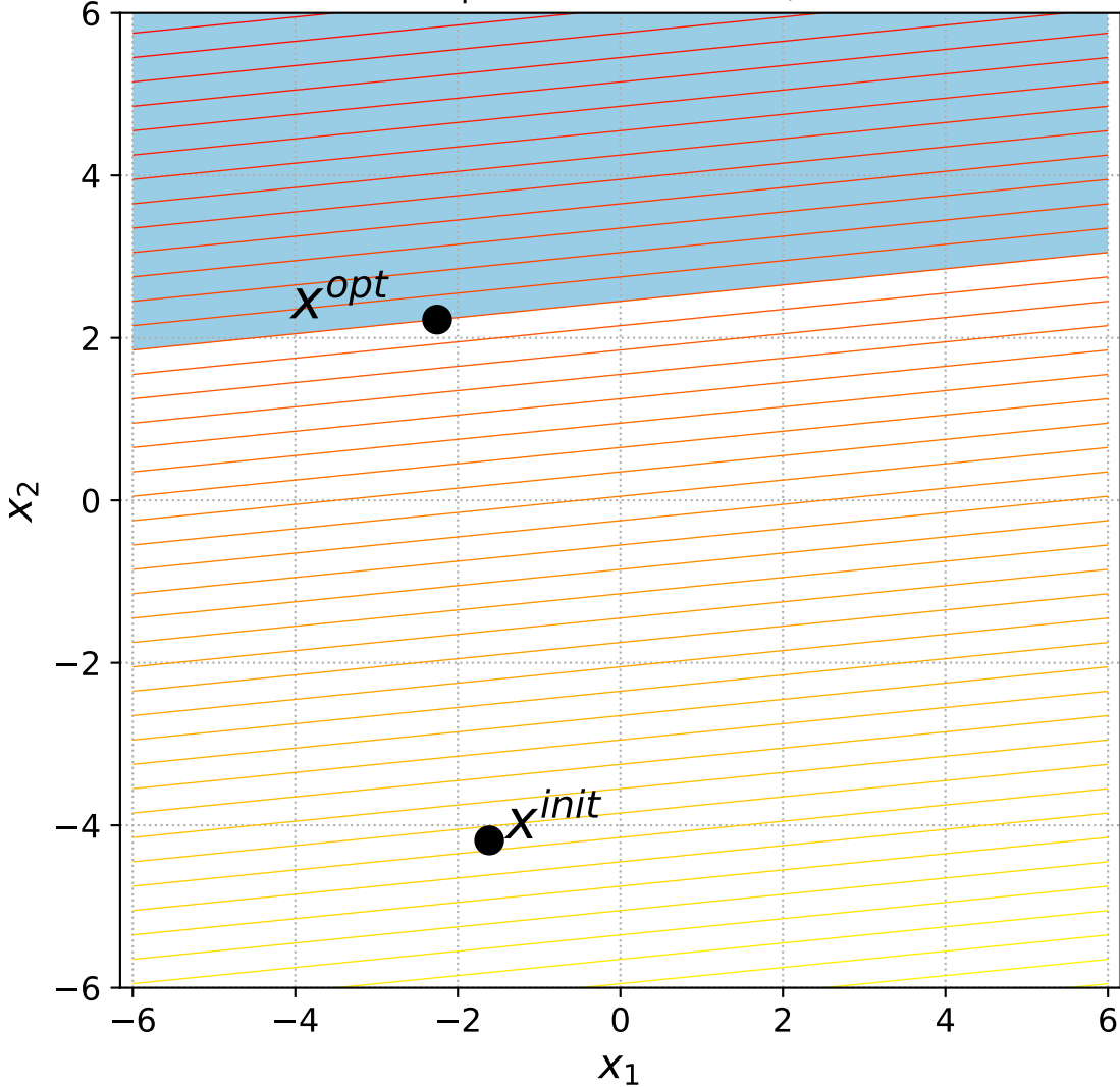
13 Linear Slope with 1 constraint, instance=8
