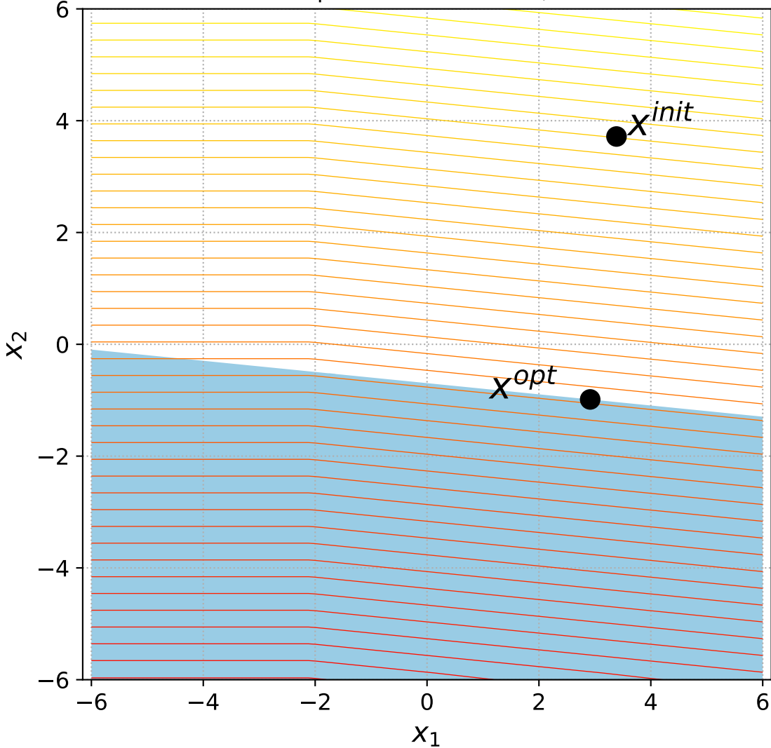
13 Linear Slope with 1 constraint, instance=7
