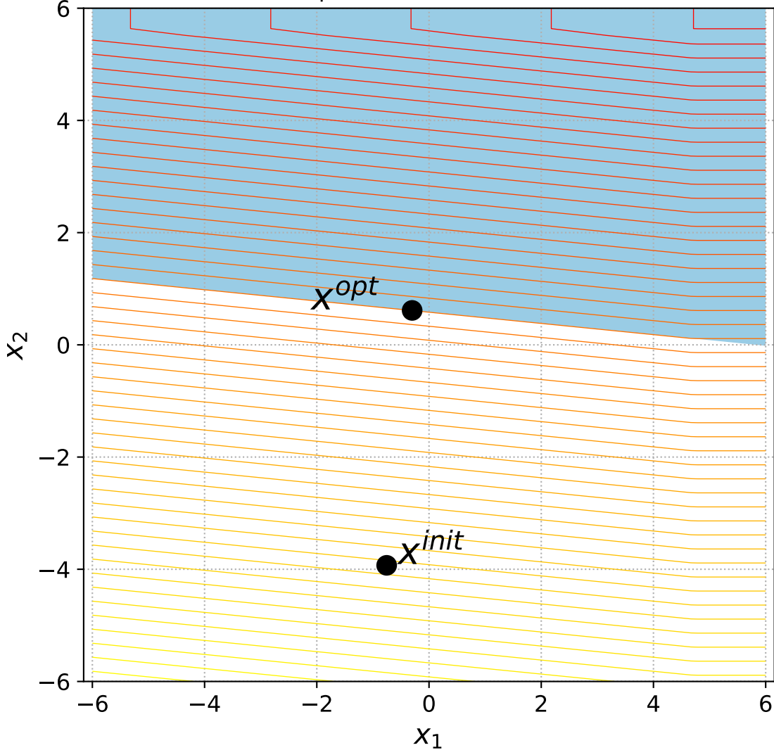
13 Linear Slope with 1 constraint, instance=6
