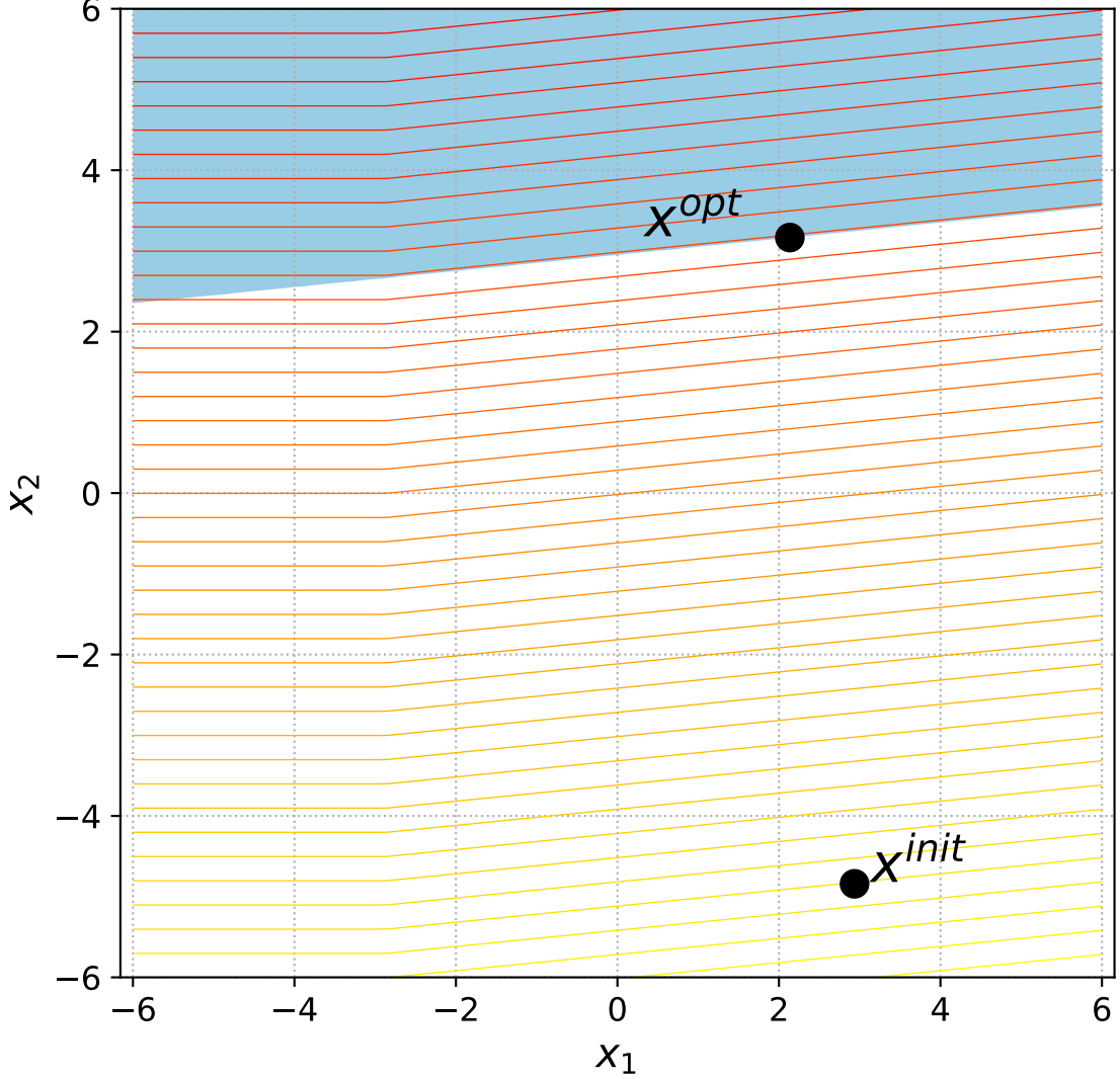
13 Linear Slope with 1 constraint, instance=5
