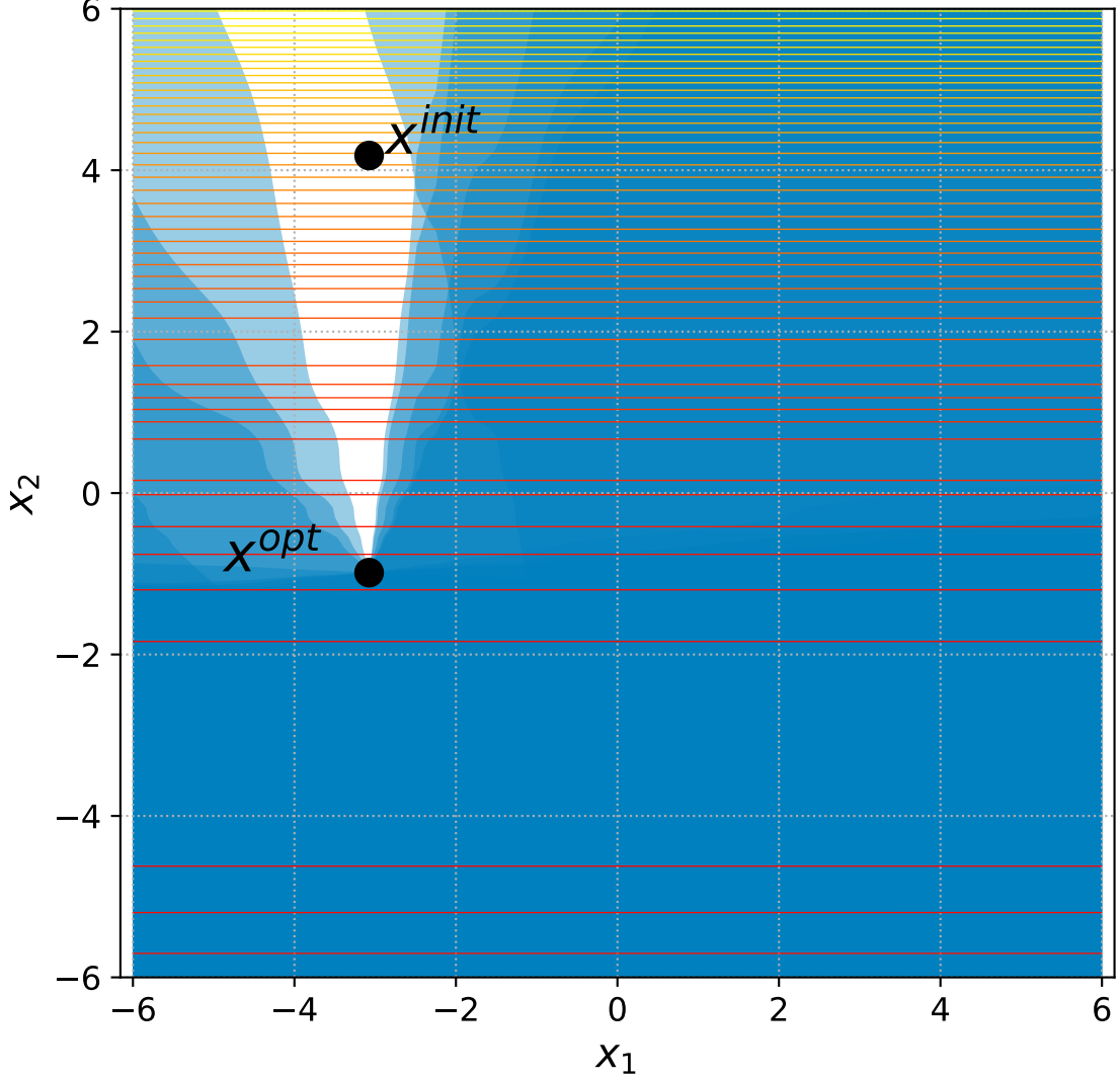
12 Sep. Ellipsoid with 6+3n constraints, instance=15
