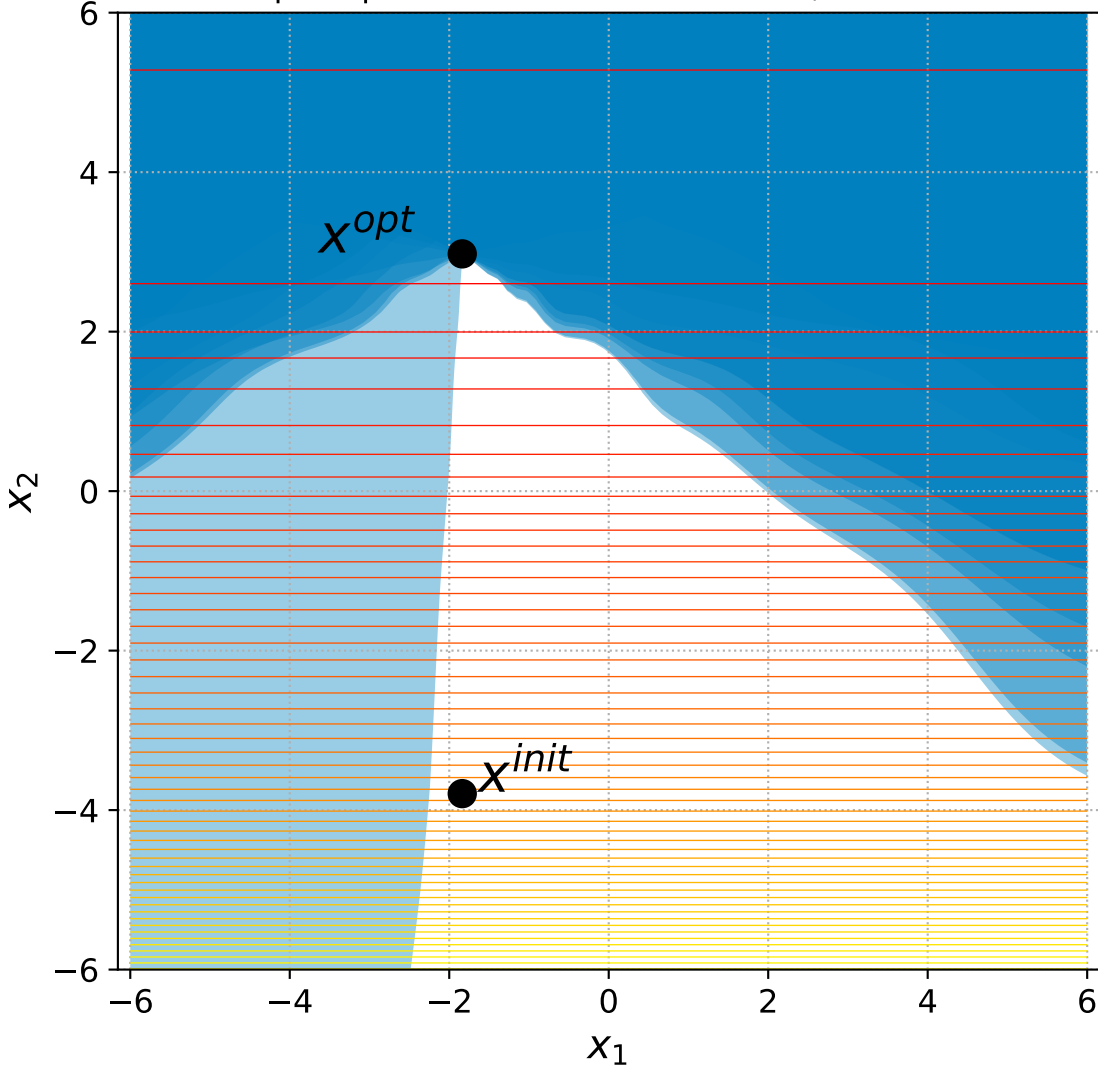
12 Sep. Ellipsoid with 6+3n constraints, instance=14
