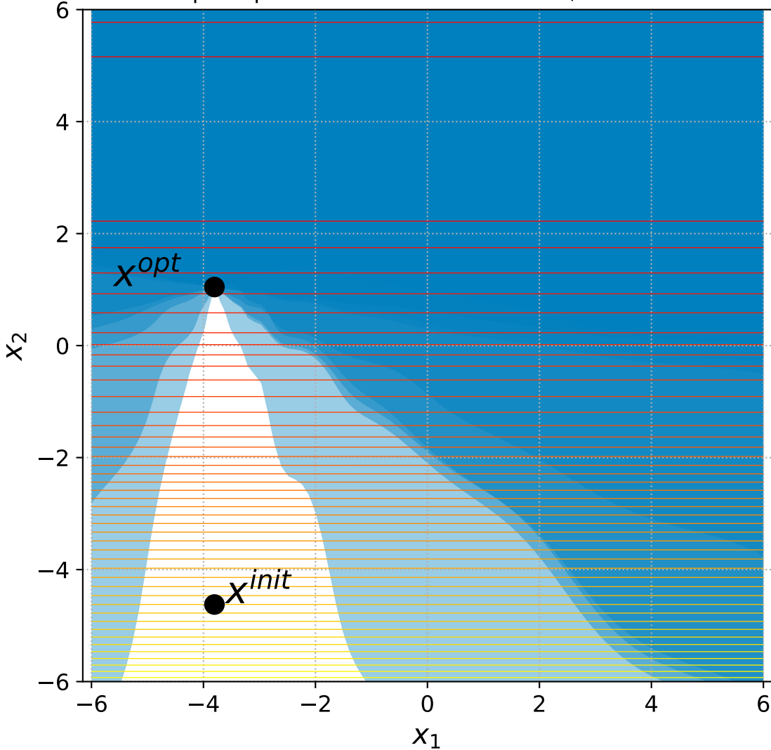
12 Sep. Ellipsoid with 6+3n constraints, instance=12
