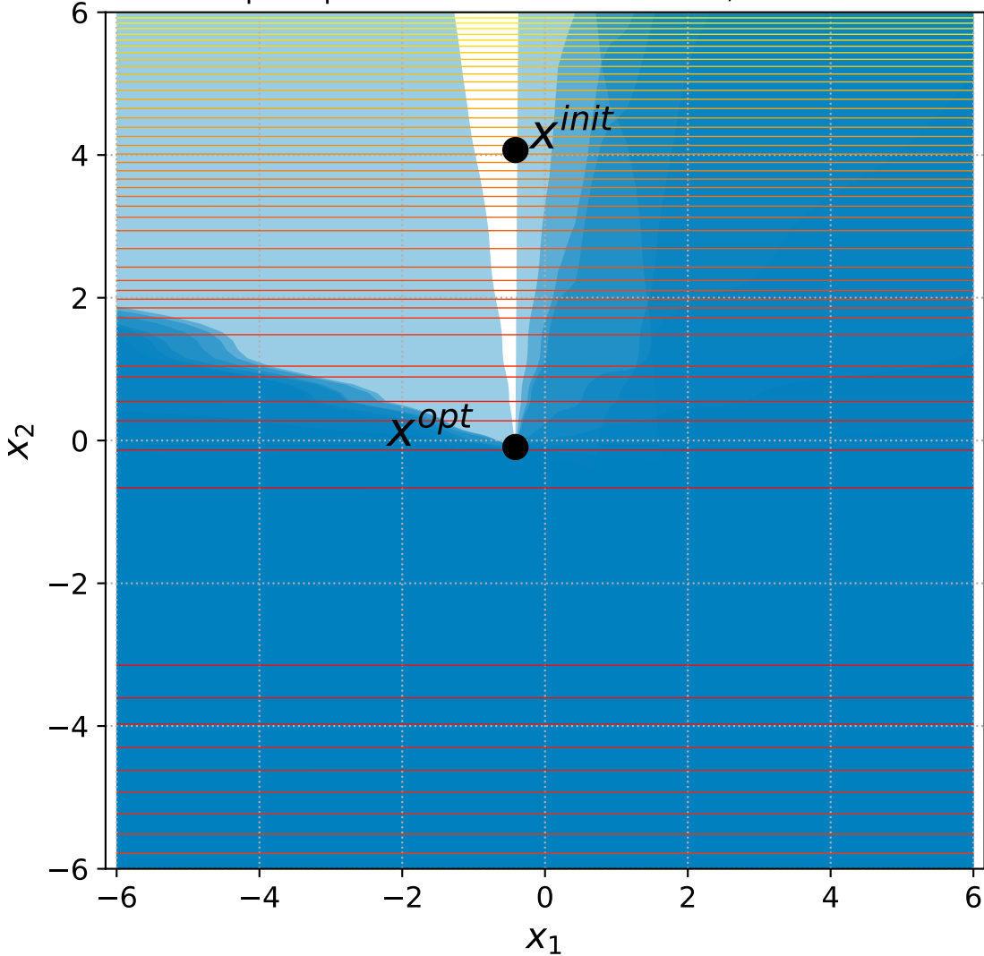
12 Sep. Ellipsoid with 6+3n constraints, instance=11
