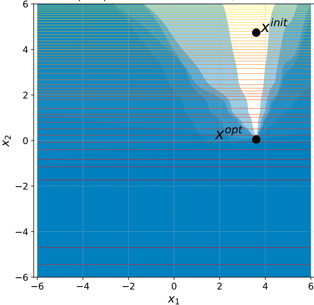
12 Sep. Ellipsoid with 6+3n constraints, instance=10
