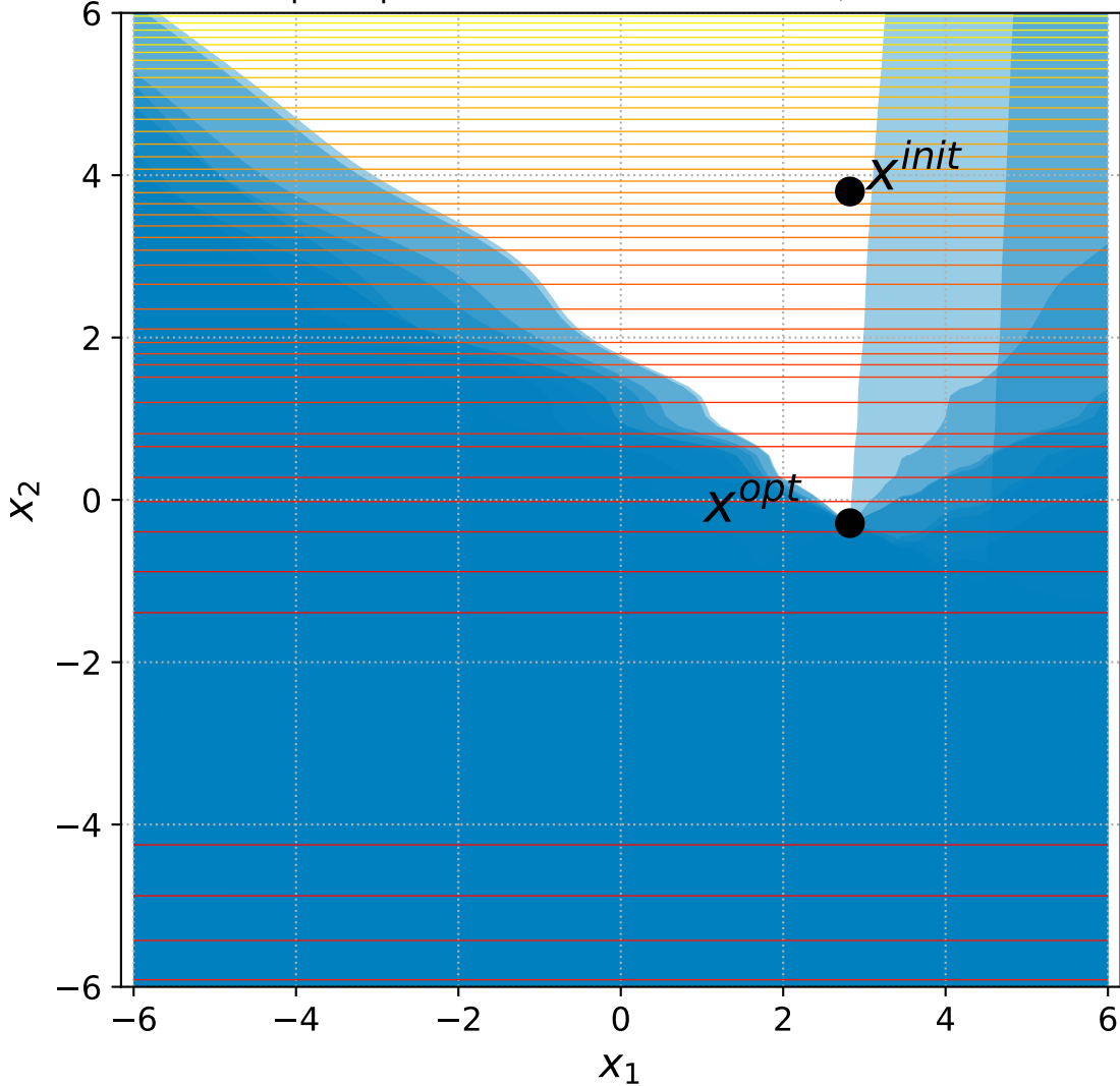
12 Sep. Ellipsoid with 6+3n constraints, instance=9
