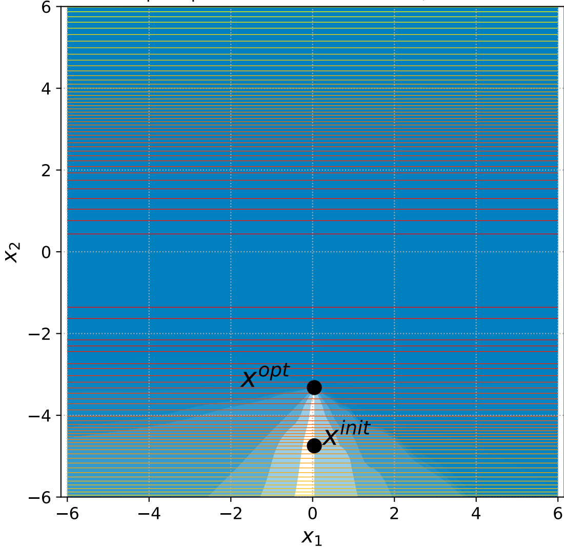
12 Sep. Ellipsoid with 6+3n constraints, instance=8
