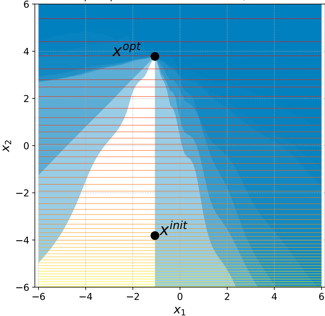
12 Sep. Ellipsoid with 6+3n constraints, instance=3
