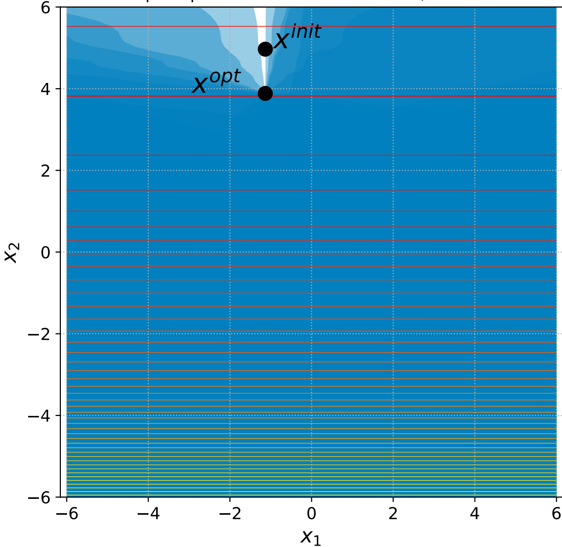
12 Sep. Ellipsoid with 6+3n constraints, instance=1
