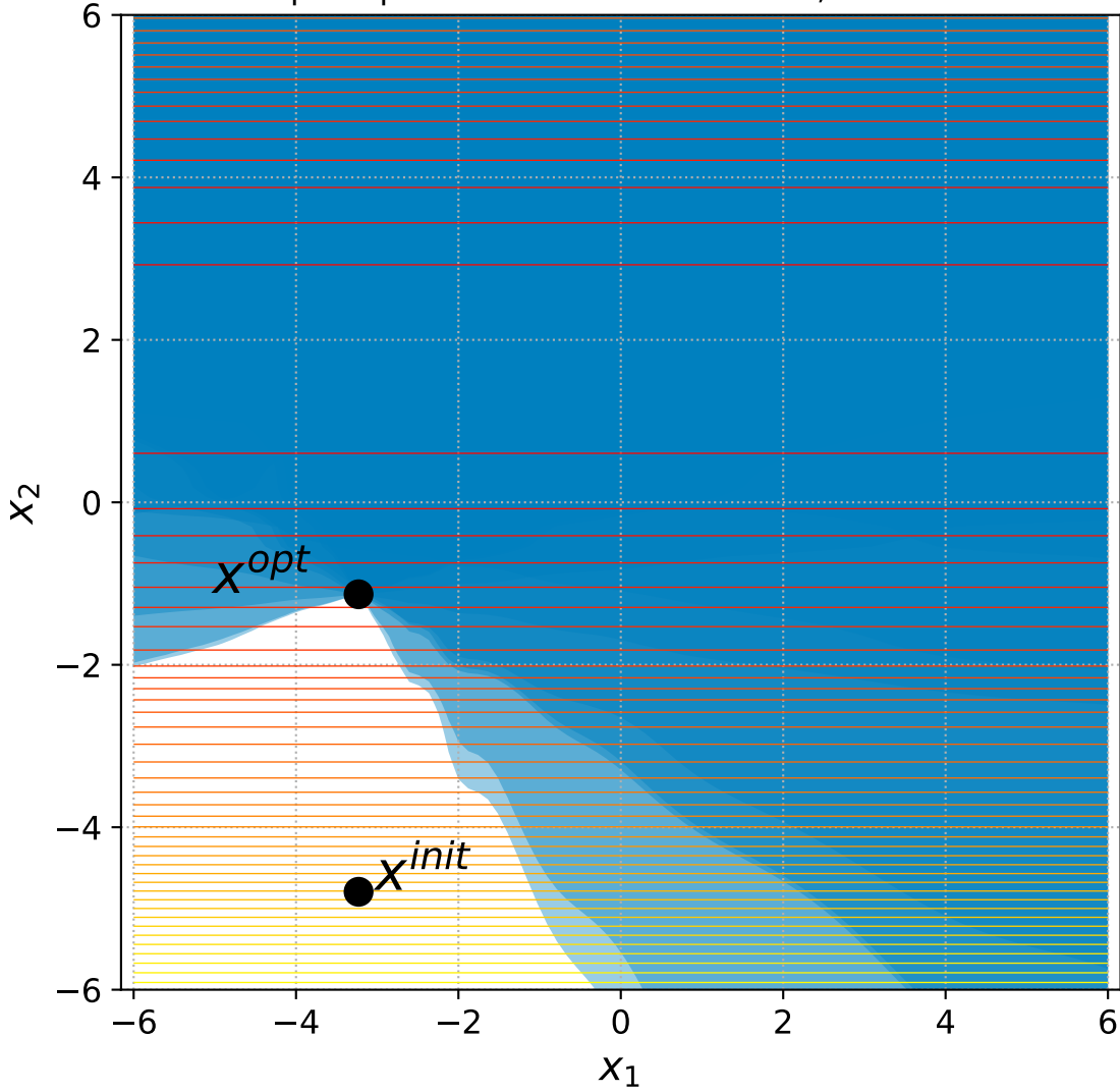
11 Sep. Ellipsoid with 6+n constraints, instance=14
