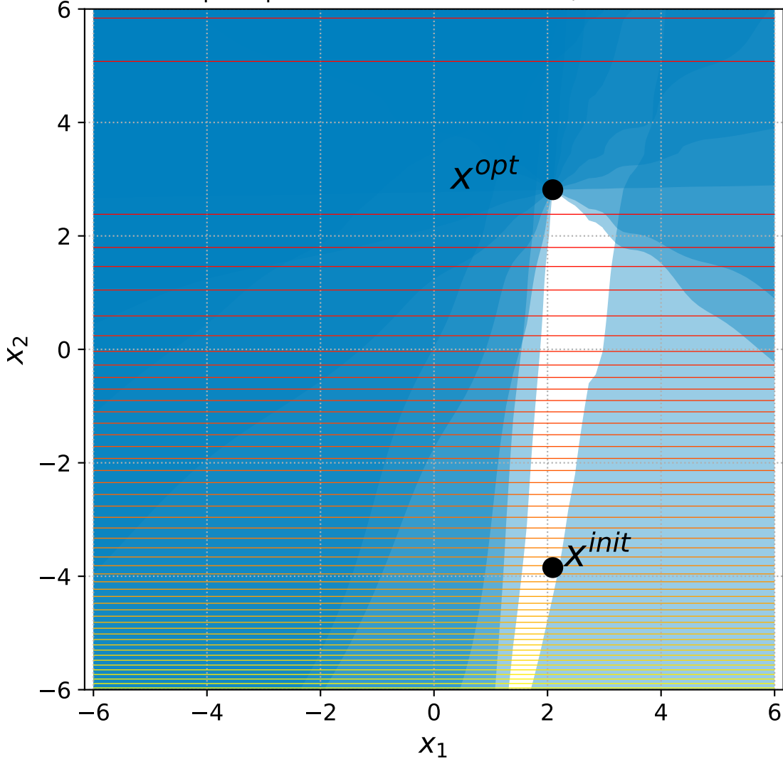
11 Sep. Ellipsoid with 6+n constraints, instance=13
