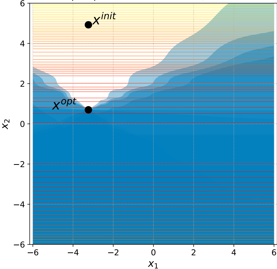
11 Sep. Ellipsoid with 6+n constraints, instance=12
