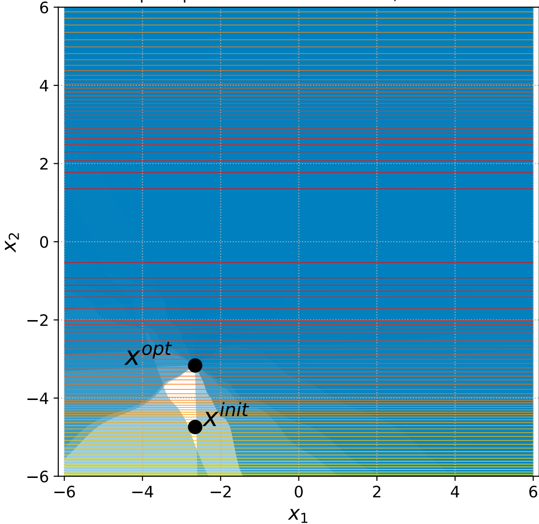
11 Sep. Ellipsoid with 6+n constraints, instance=11
