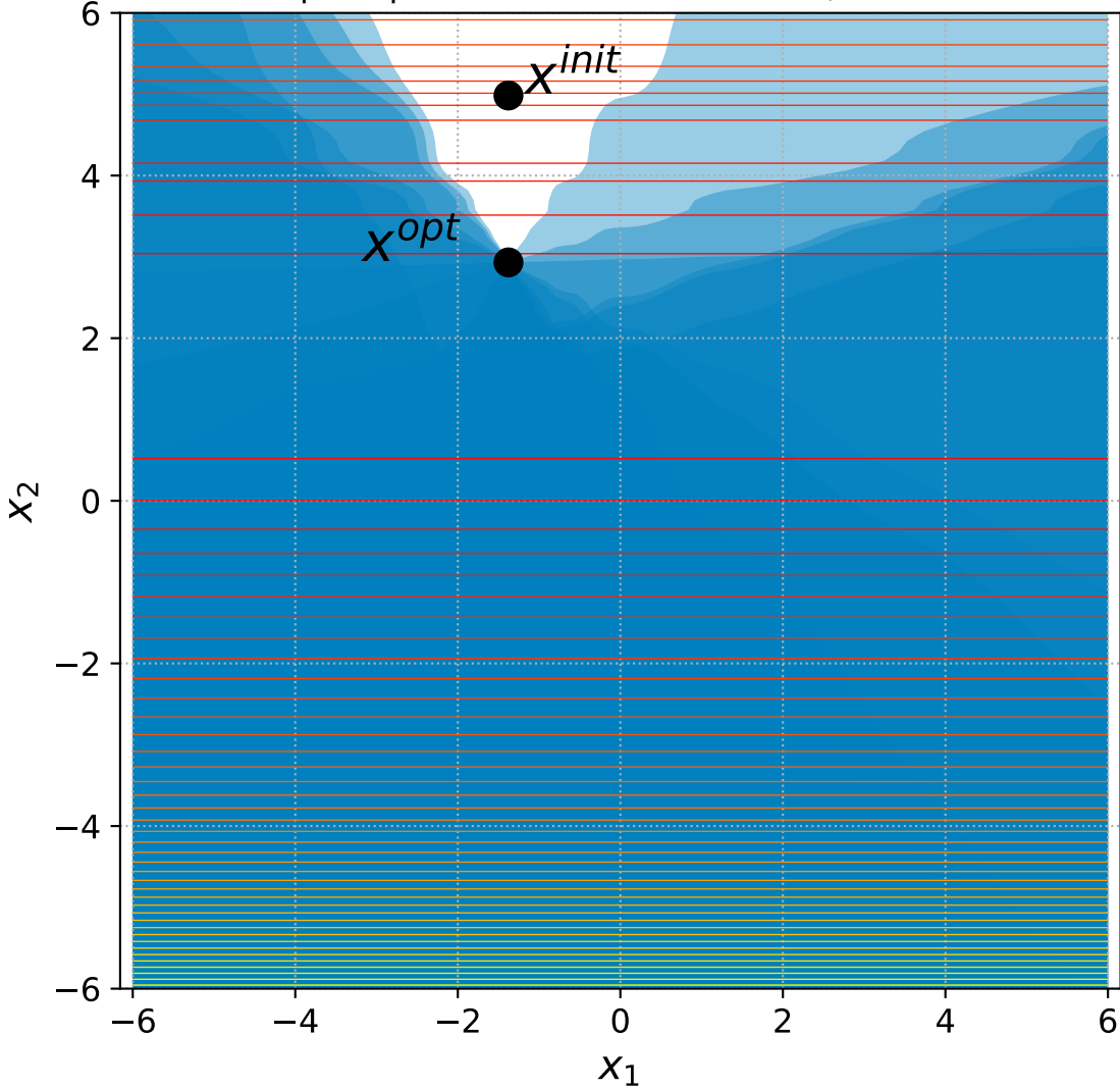
11 Sep. Ellipsoid with 6+n constraints, instance=9
