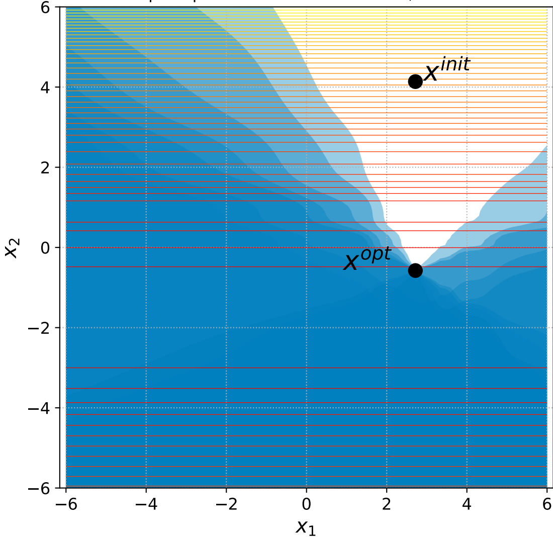
11 Sep. Ellipsoid with 6+n constraints, instance=7
