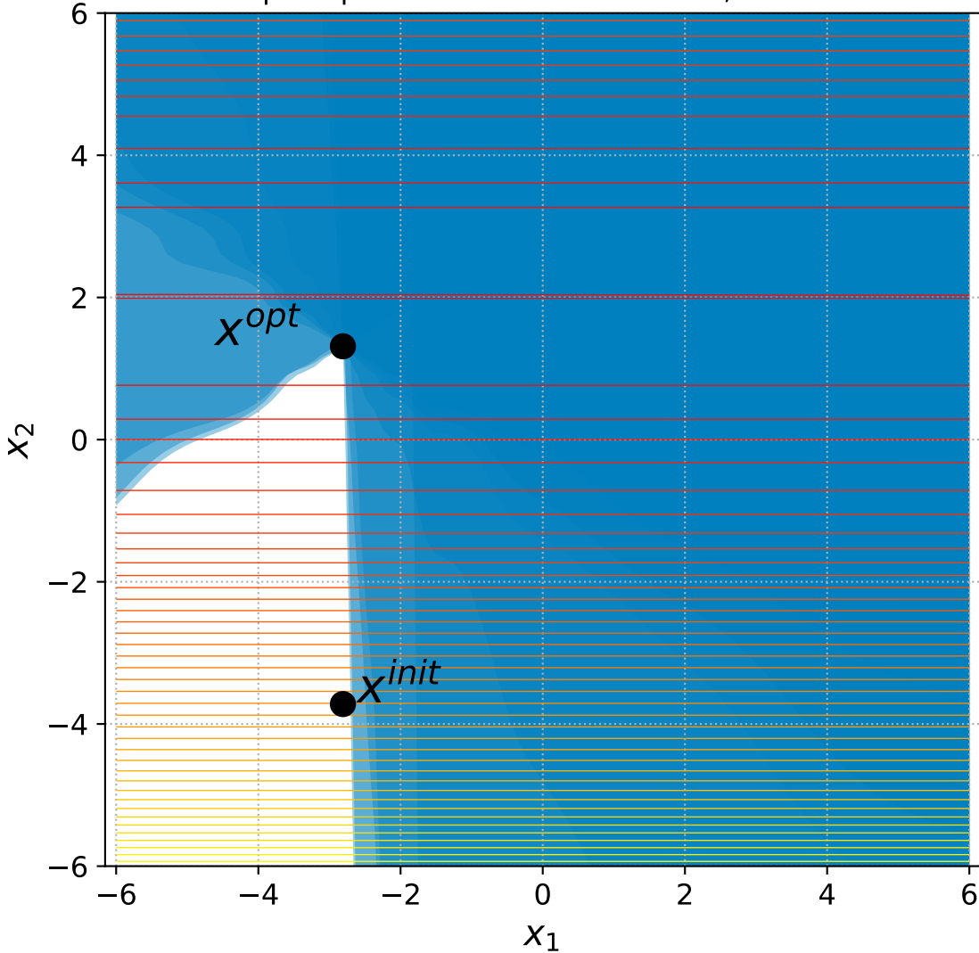
11 Sep. Ellipsoid with 6+n constraints, instance=6
